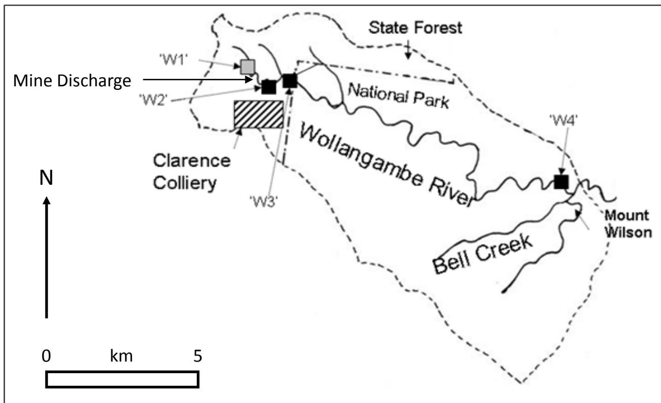
Figure 1. Map of stream sampling sites, waterways and waste discharge point in the upper Wollangambe River. Approximate catchment boundary is dashed line. Gray symbol represents the upstream reference site (W1) and black symbols the sampling sites (W2 to W4) on the Wollangambe River below the coal mine waste discharge. The Blue Mountains National Park/State Forest Boundary is indicated.
